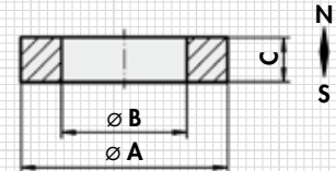
Ring magnets MK 52:
